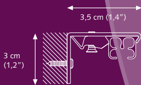
Wall bracket
