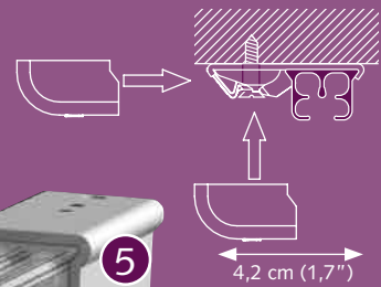
Ceiling Bracket
